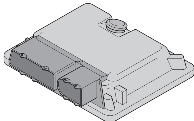
Engine control unit, 80-pin connector
